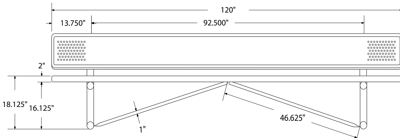
front
