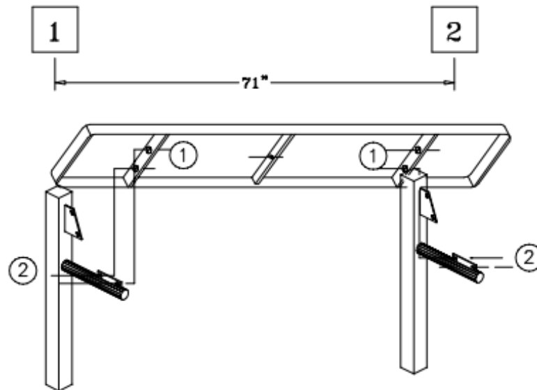
FOOTING DIAGRAM:
