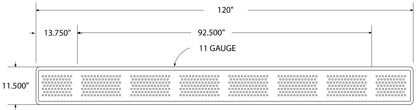
top view
