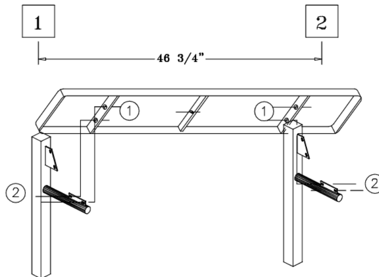
FOOTING DIAGRAM:
